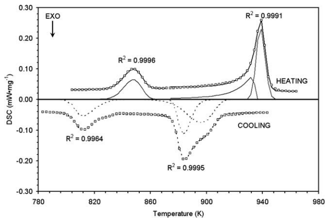
Fig. 7. Deconvoluted differential scanning calorimetry trace for Alloy-A. The anticipated transitions (3) could be reasonably separated from the experimental data with correlation coefficients listed on the figure.
