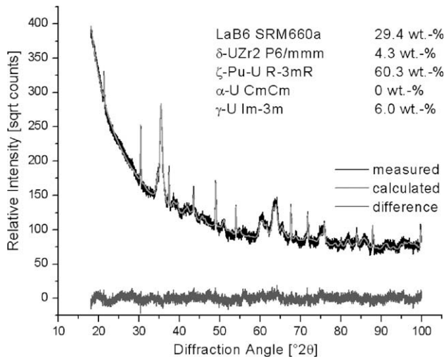
Fig. 5. Example of a refined Rietveld diffraction pattern for Alloy-A. Note the peaks from 60–66° 2 \theta that are characteristic of the \zeta -phase.
