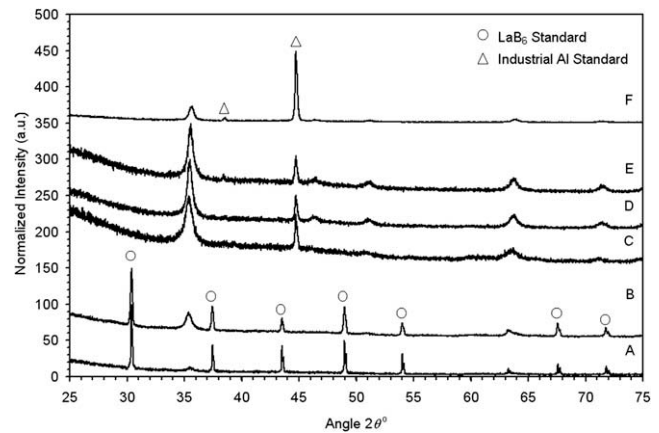
Fig. 4. X-ray diffraction patterns for the AFC-1 and AFC-2 metallic fuel alloys measured with either LaB 6 (SRM 660a) or industrial Al internal standard. Alloy-A is at the bottom, and alloys progress accordingly to F at the top.
